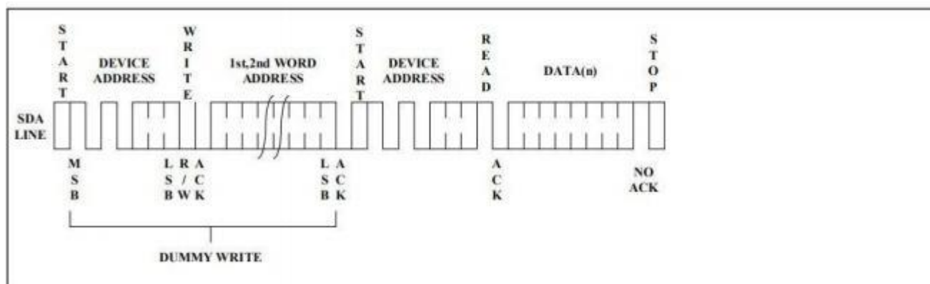
Figure 9. Random Read
