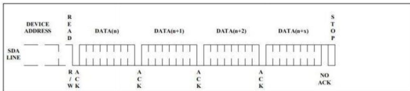
Figure 10. Sequential Read
