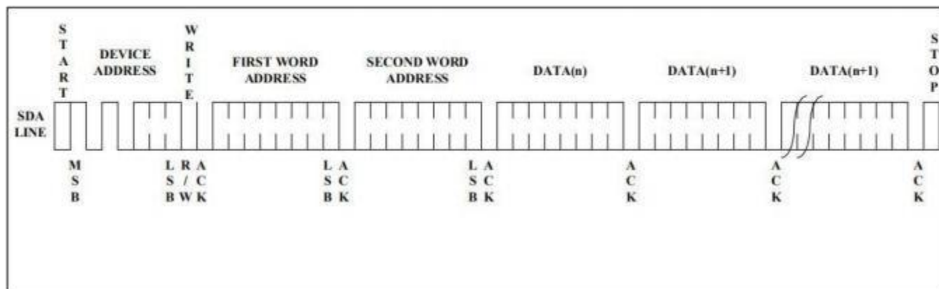
Figure 7. Page Write
